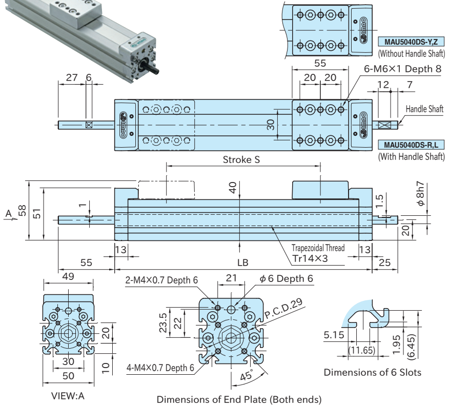
Dimensions of End Plate (Both ends)
